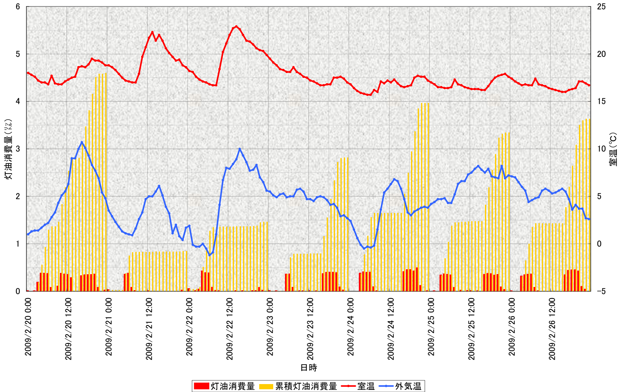
Graph1 (2) 灯油消費量と室温
