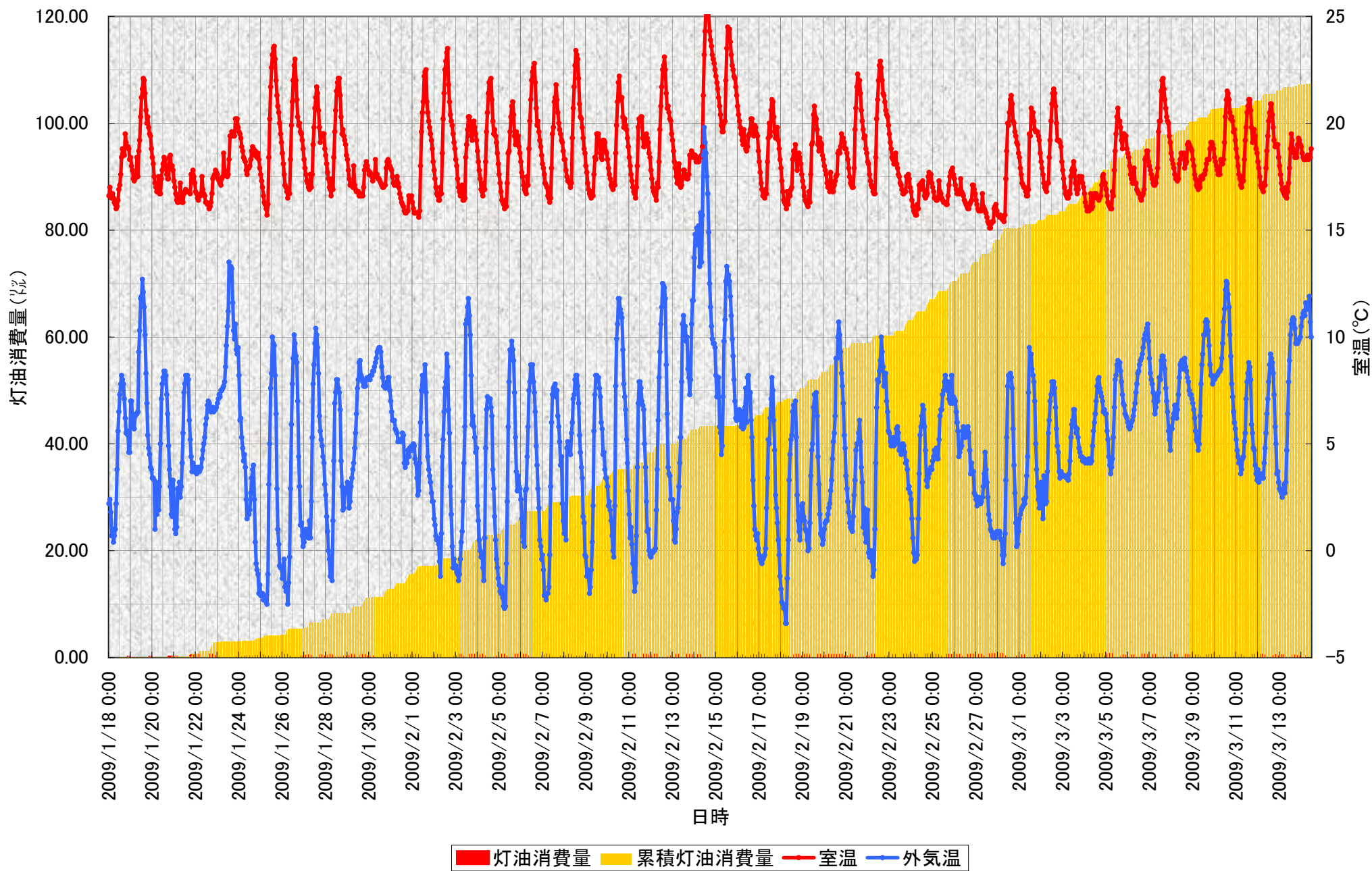
Graph1 灯油消費量と室温
